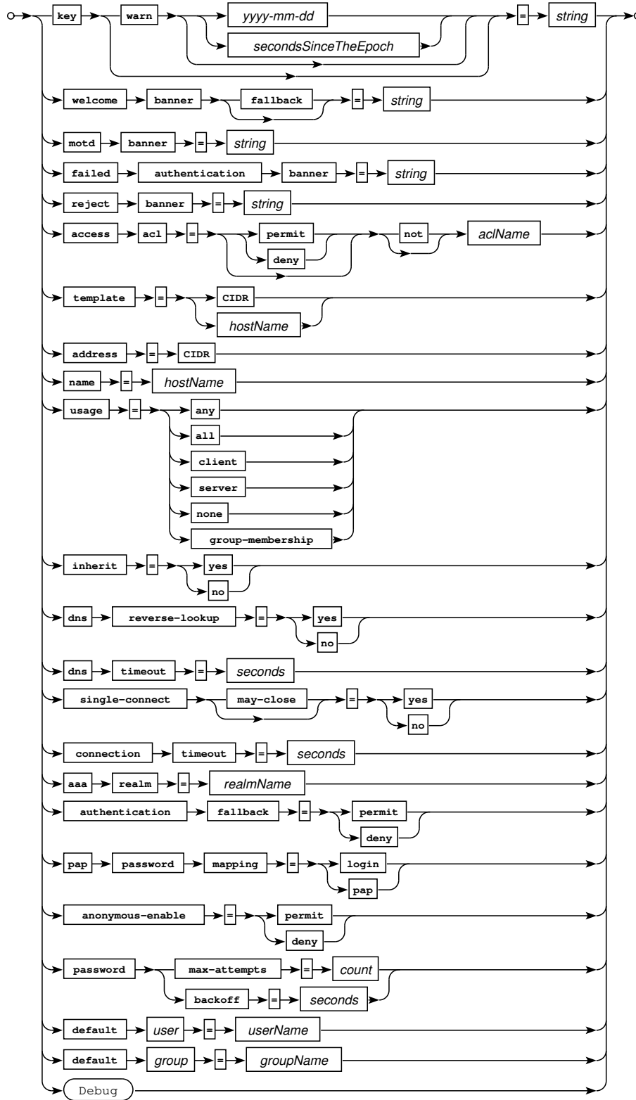
Railroad diagram: HostAttr
